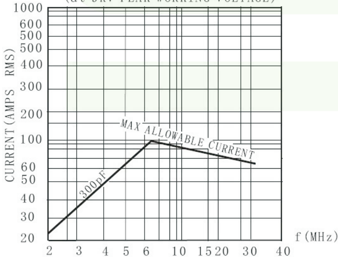
CONTINUOUS RMS AMPERES VS FREQUENCY (at 9kV PEAK WORKING VOLTAGE)
