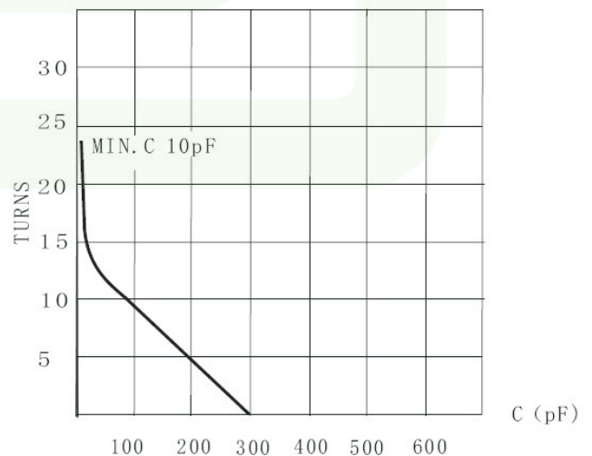
CAPACITY vs TURNS Typical Data
