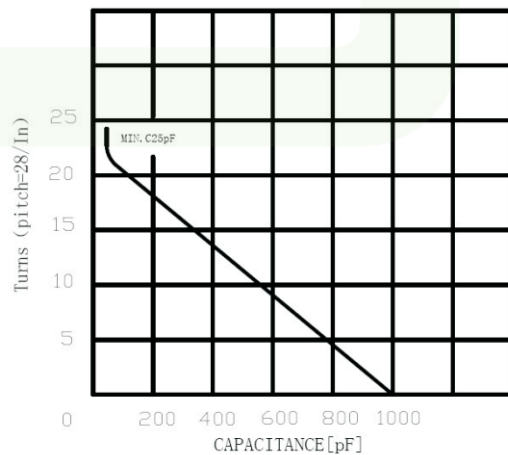
CAPACITY vs TURNS Typical Data
